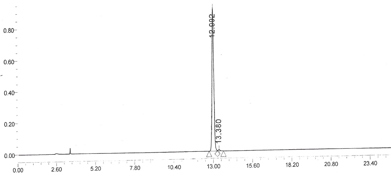
Auto-Scaled Chromatogram
